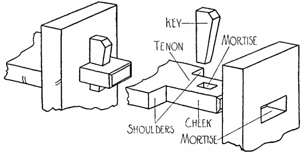
FIG. 254. KEYED MORTISE-AND-TENON JOINT.
